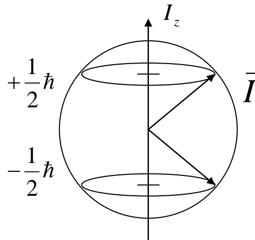
Spin 1/2 example
